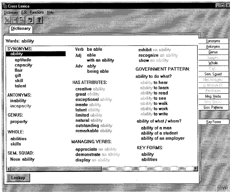
Figure 1. Screenshot of CrossLexica
