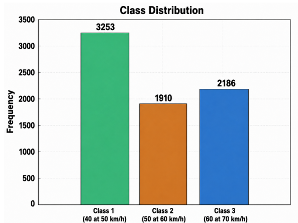
Fig. 2. Class distribution
